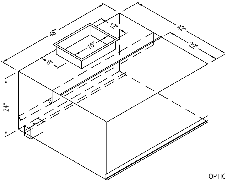
ISOMETRIC
